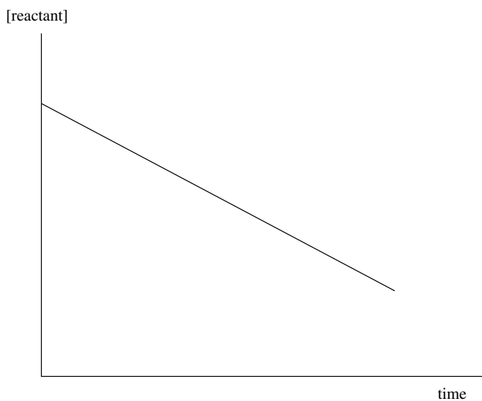
Figure 3.2 Graph of [\text{reactant}] versus time showing linearity
