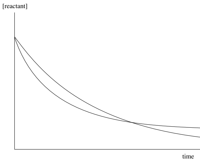
Figure 3.1 Graphs of [\text{reactant}] versus time showing curvature
